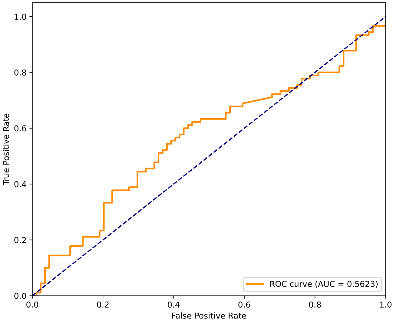
ROC Curve - SVM_Linear
